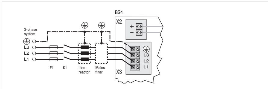
Illustration 23.2 BG4 mains supply connection 1 x 230 V
