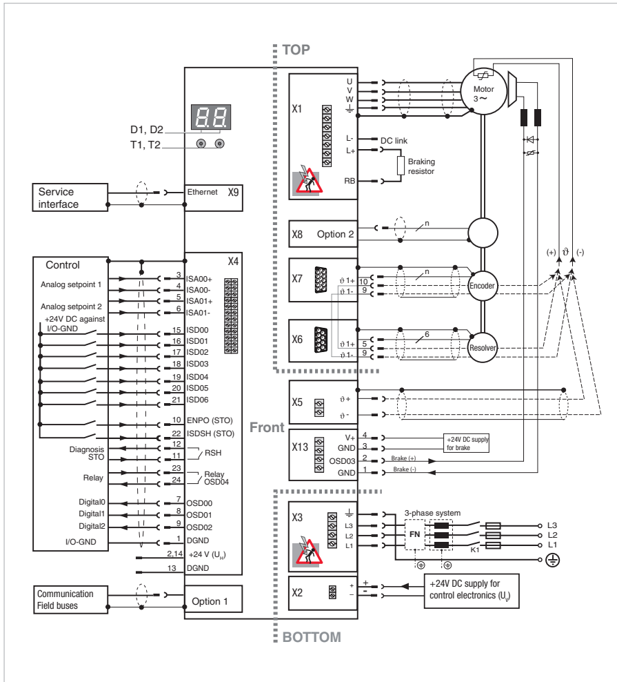
Illustration 14.2 Connection diagram
