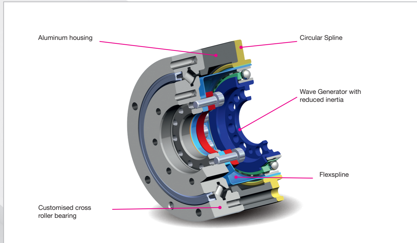
Lightweight gear based on CPL-2A Gear Component Set
