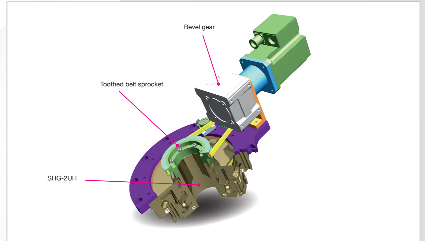
Swivel joint for X-ray system based on the SHG-2UH Hollow Shaft Gear, bevel gear pre-stage and a toothed belt pre-stage
