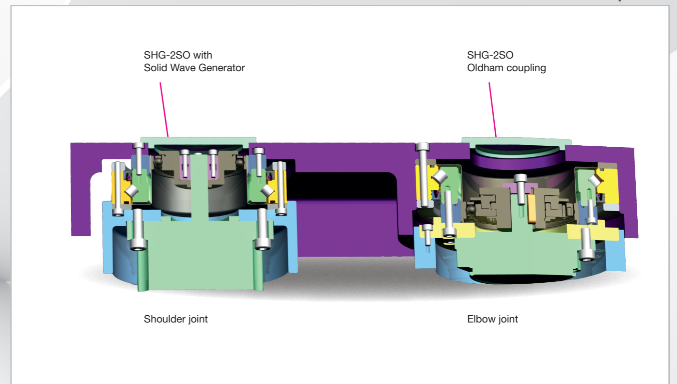
Two SCARA robot axes based on SHG-2SO with motor adaptation
