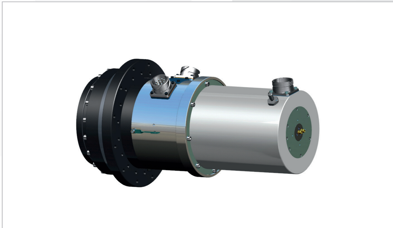
AlopexDrive Actuator including slip ring and fibre optic cable
