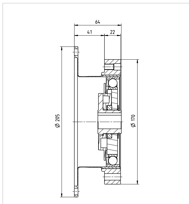
HFUS-50-2A [mm]
