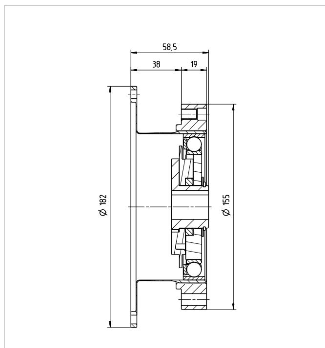
HFUS-45-2A [mm]
