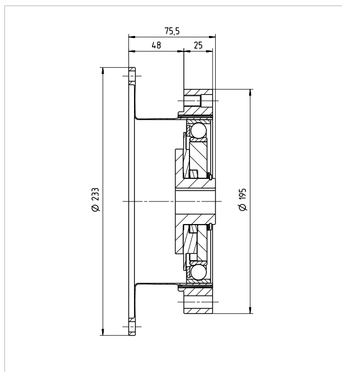
SHG-58-2A [mm]
