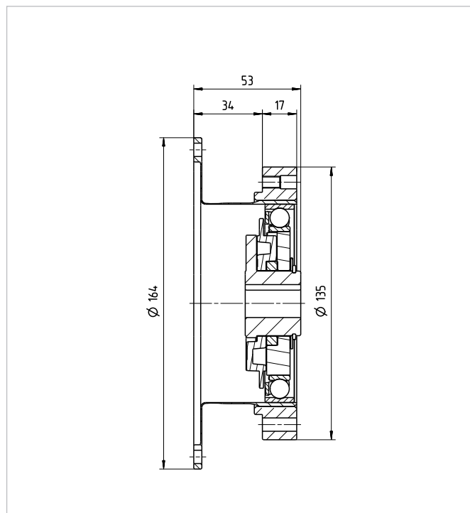
HFUS-40-2A [mm]
